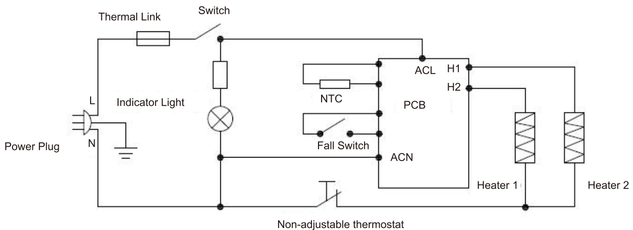
Figure 5 Product Electrical Schematic Diagram
